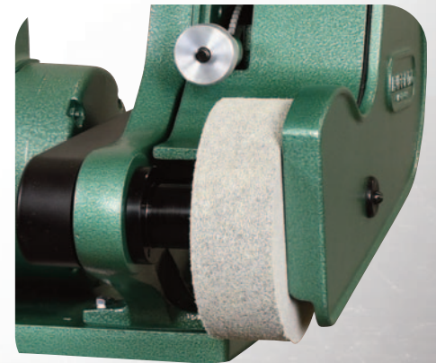
Easily mount surface conditioning wheels up to 2" wide with available wheel adapters.
